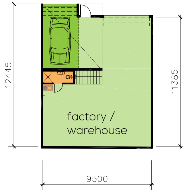
lower ground floor plan
